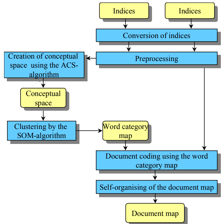
Figure 6: Overview of the ACS-WEBSOM-algorithm
